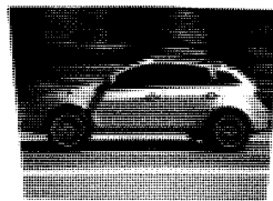
9 car
