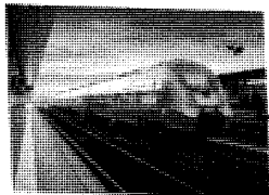
0 train
