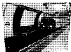
2 underground
