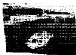
6 boat
