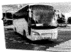
5 coach
