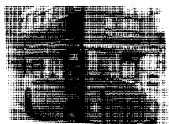
7 bus
