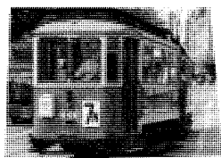
1 tram
