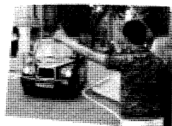
8 taxi
