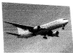
4 plane
