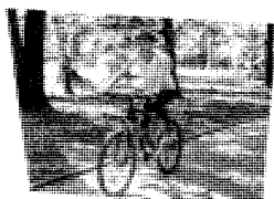
3 bike
