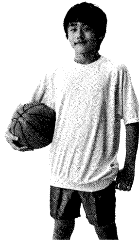
1 tom
